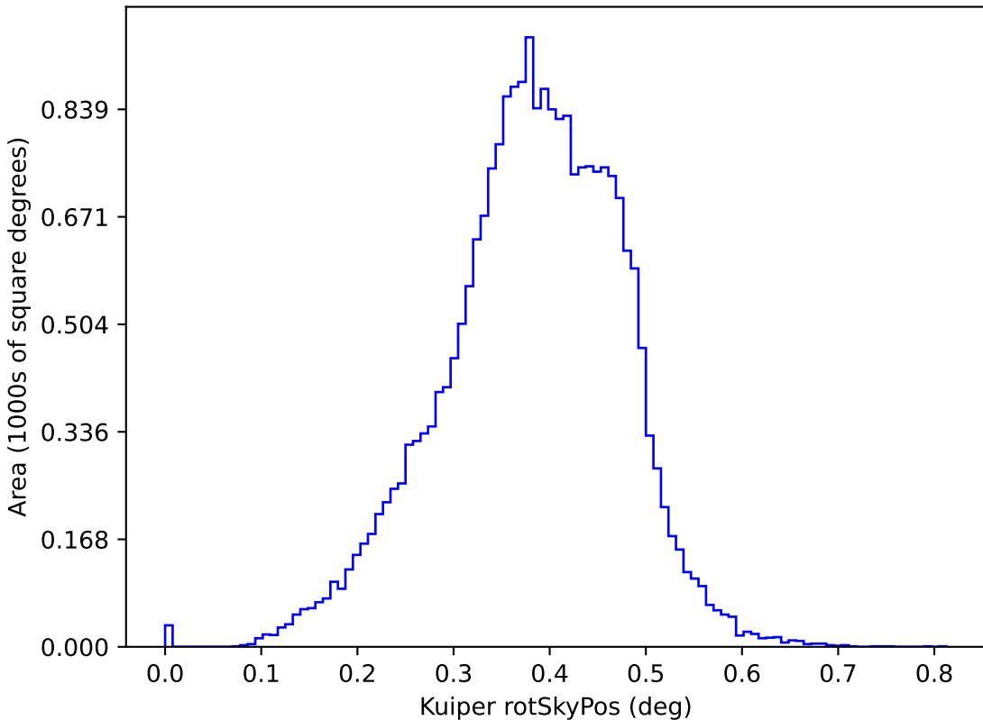
ddf_loaded_half_fl15_v3.3_10yrs y: Kuiper rotSkyPos
