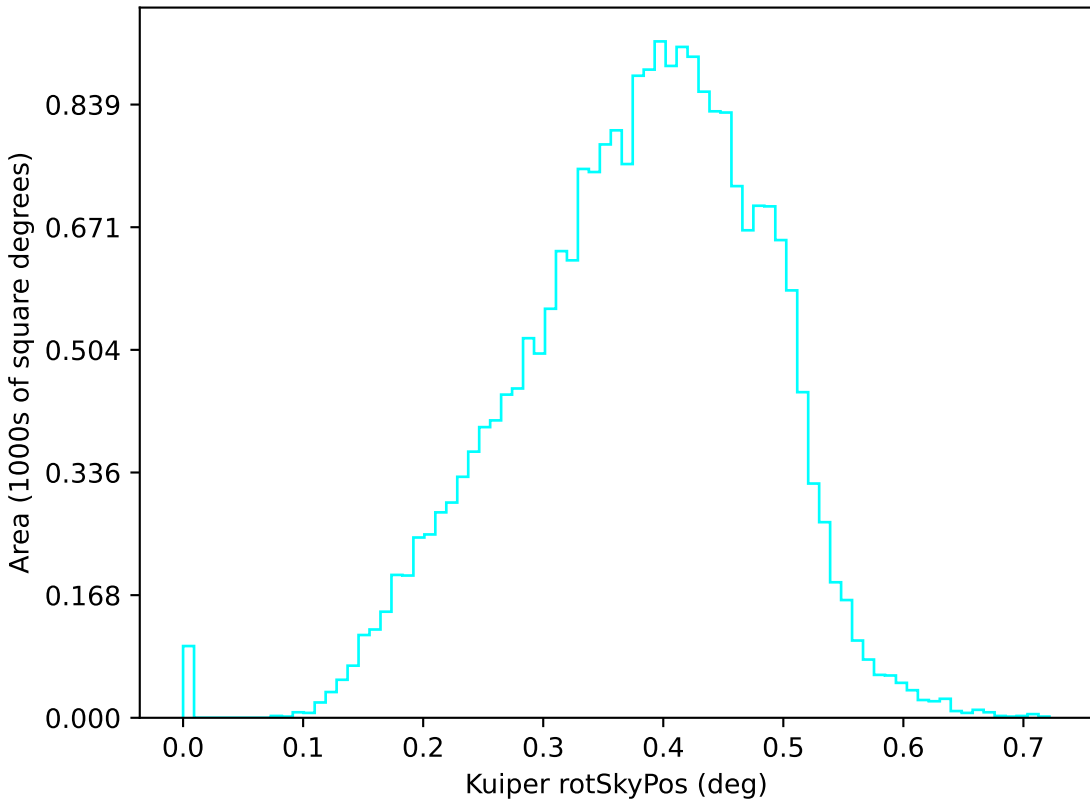
ddf_loaded_half_fl15_v3.3_10yrs u: Kuiper rotSkyPos
