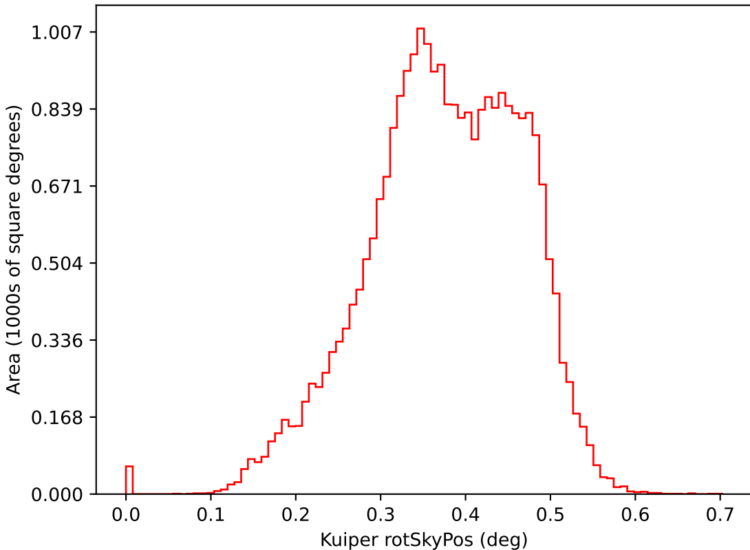
ddf_loaded_half_fl15_v3.3_10yrs i: Kuiper rotSkyPos
