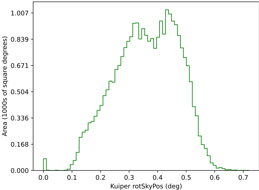
ddf_loaded_half_fl15_v3.3_10yrs g: Kuiper rotSkyPos
