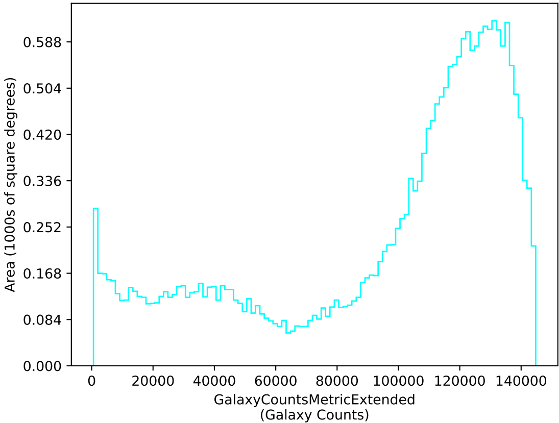
ddf_loaded_half_fl15_v3.3_10yrs u: GalaxyCountsMetricExtended
