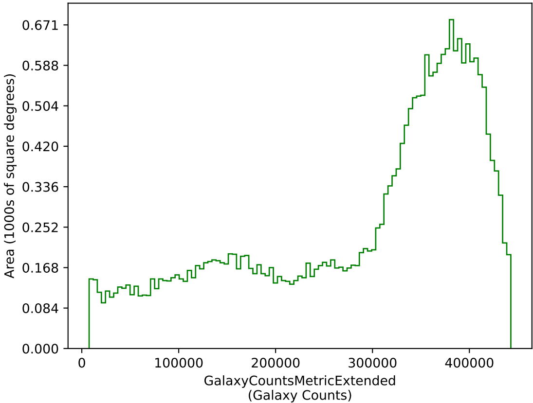
ddf_loaded_half_fl15_v3.3_10yrs g: GalaxyCountsMetricExtended
