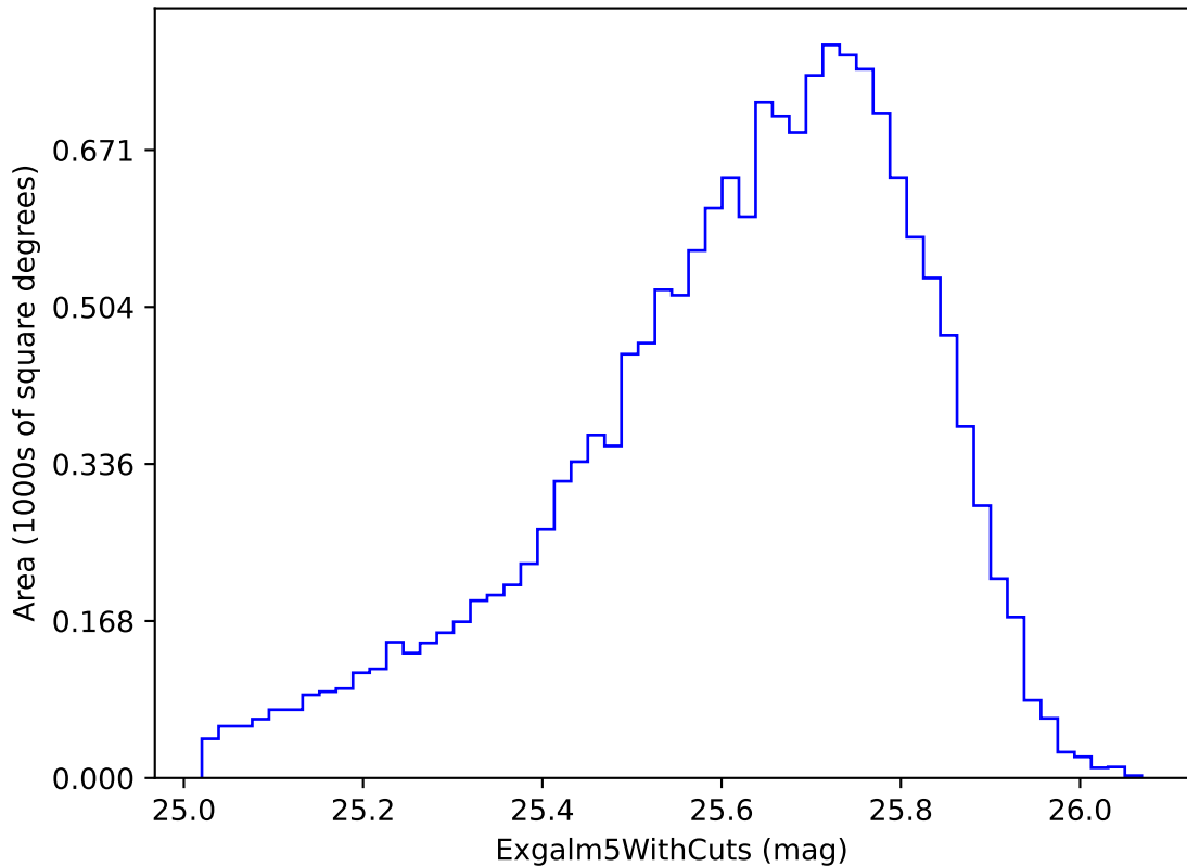
ddf_loaded_half_fl15_v3.3_10yrs i band non-DD year 2: Exgal5WithCuts
