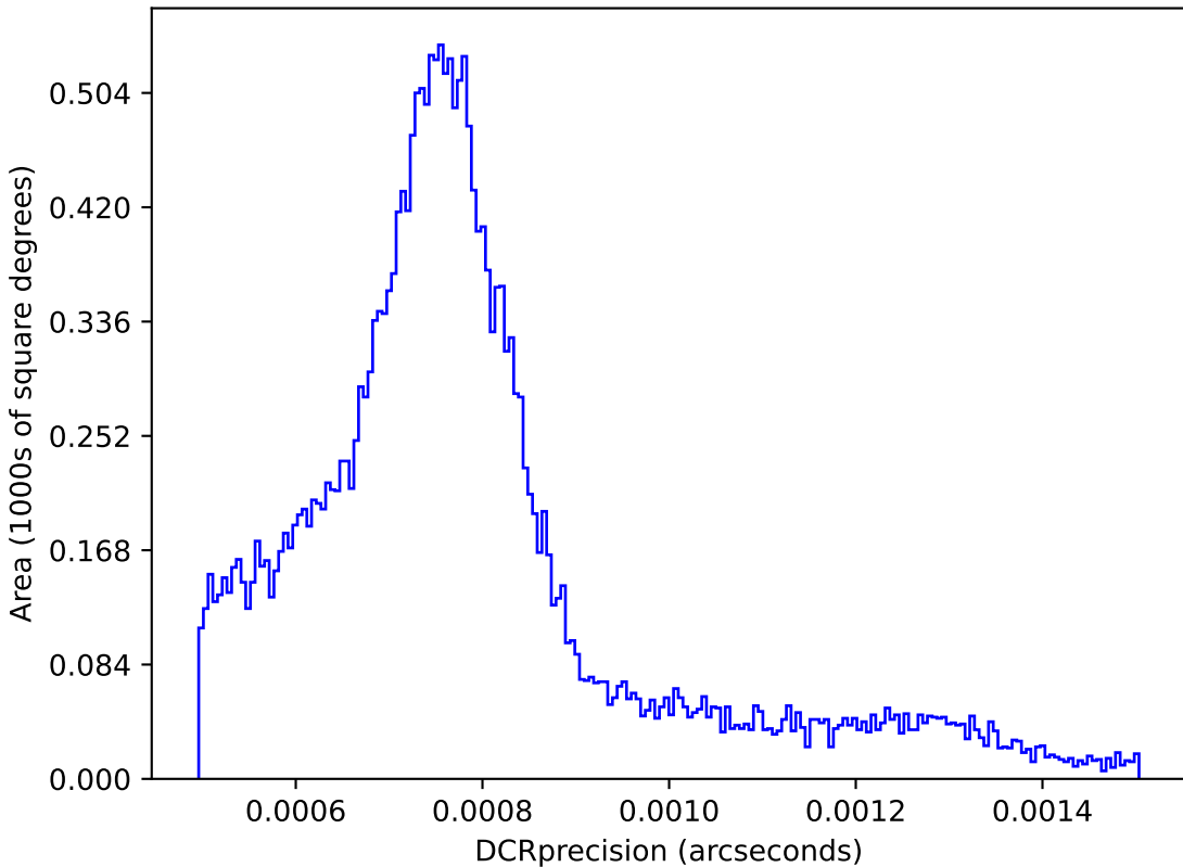
ddf_loaded_half_fl15_v3.3_10yrs : DCRprecision
