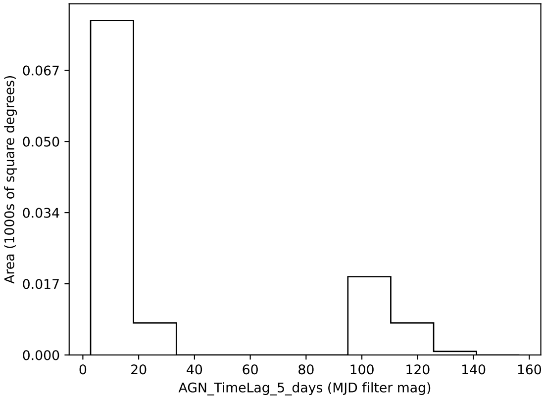
ddf_loaded_half_fl15_v3.3_10yrs all bands: AGN_TimeLag_5_days
