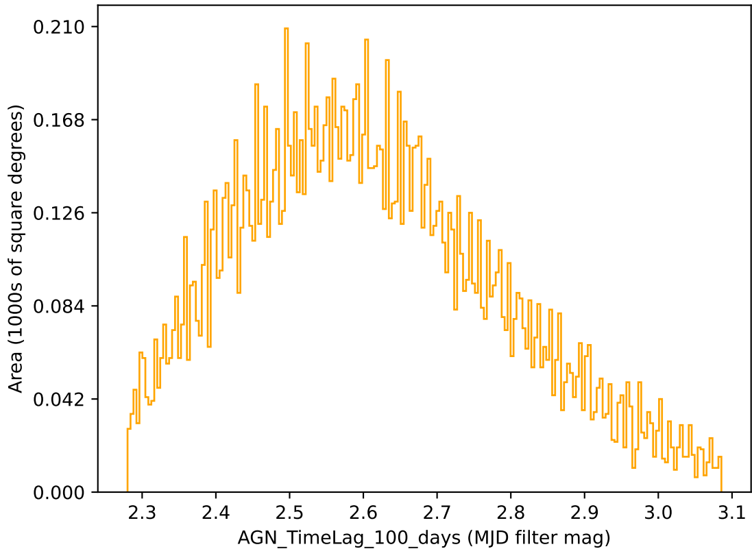
ddf_loaded_half_fl15_v3.3_10yrs r band: AGN_TimeLag_100_days
