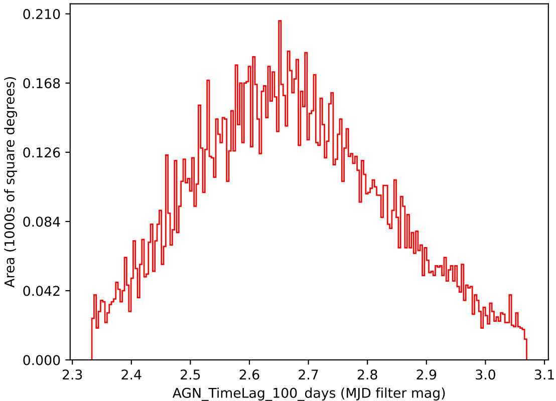
ddf_loaded_half_fl15_v3.3_10yrs i band: AGN_TimeLag_100_days
