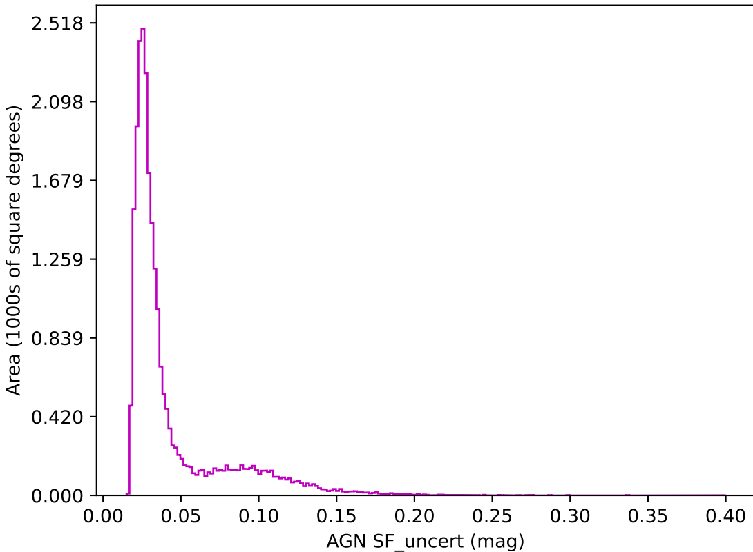
ddf_loaded_half_fl15_v3.3_10yrs z band: AGN SF_uncert
