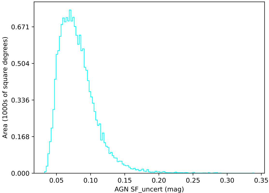
ddf_loaded_half_fl15_v3.3_10yrs u band: AGN SF_uncert
