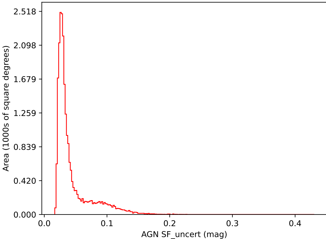
ddf_loaded_half_fl15_v3.3_10yrs i band: AGN SF_uncert
