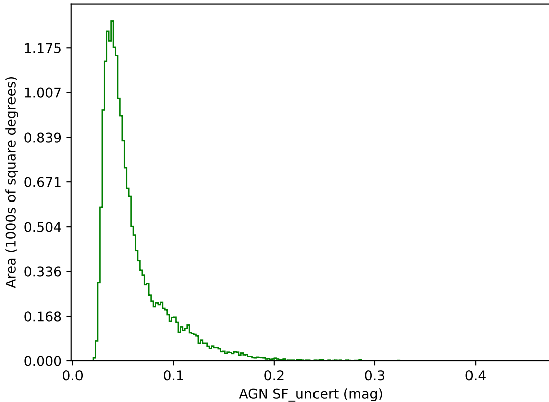
ddf_loaded_half_fl15_v3.3_10yrs g band: AGN SF_uncert
