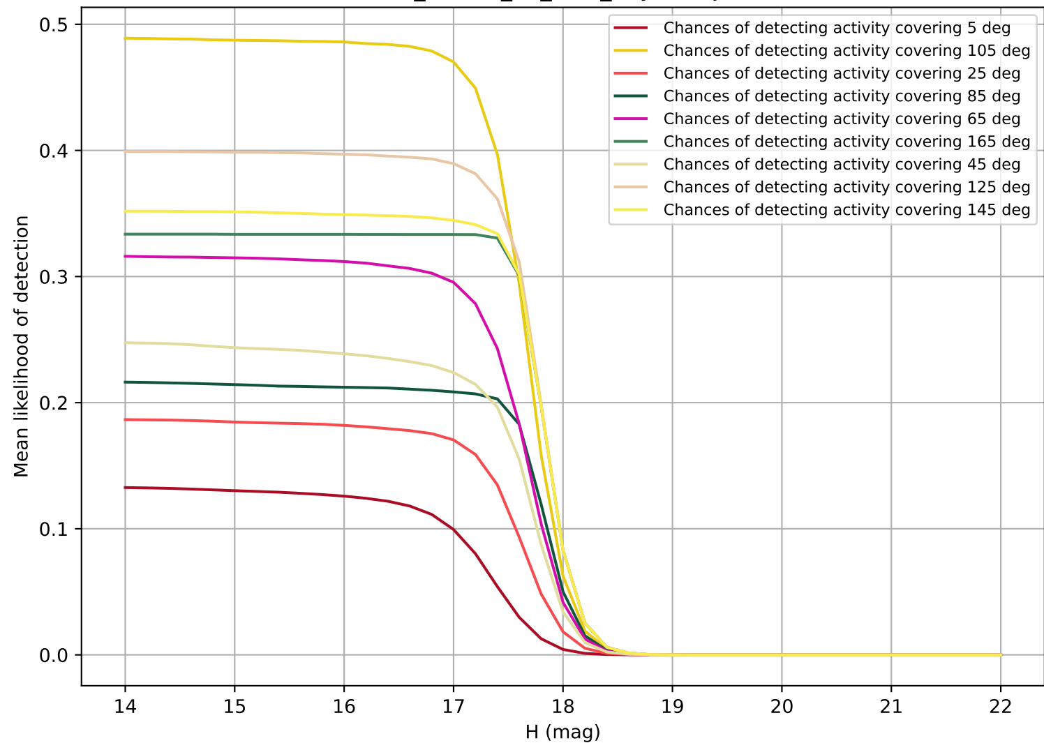
ddf_loaded_fl8_v3.4_10yrs Trojan
