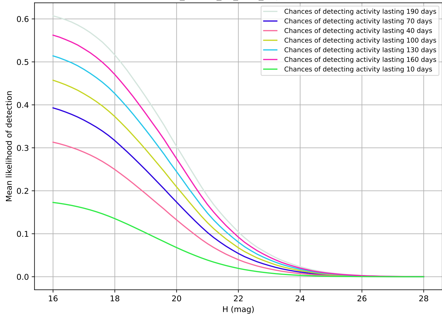
ddf_loaded_fl8_v3.4_10yrs PHA
