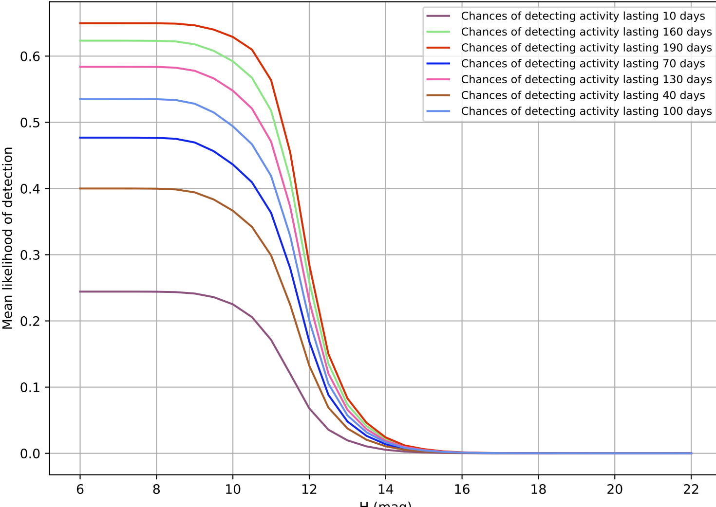
ddf loaded fl8 v3.4 10yrs OCC r20
