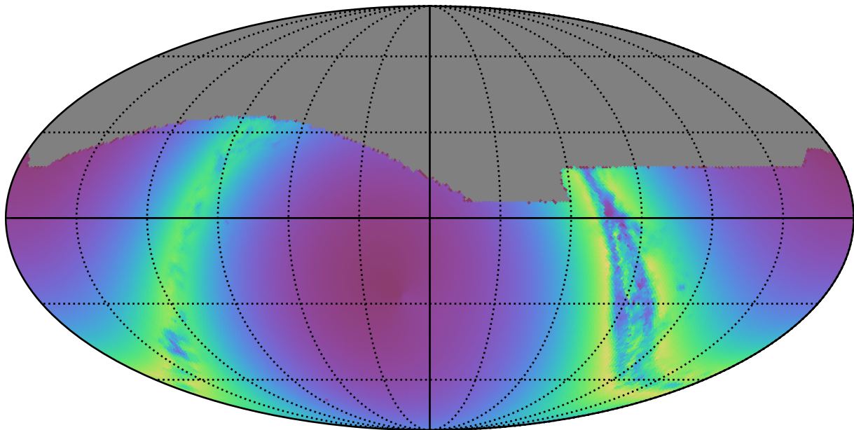
ddf_loaded_fl8_v3.4_10yrs : young_stars
