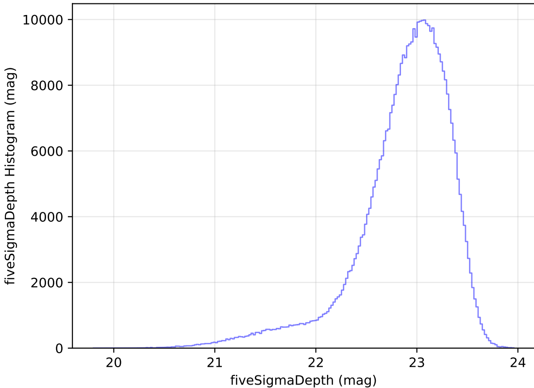
ddf_loaded_fl8_v3.4_10yrs z: fiveSigmaDepth Histogram
