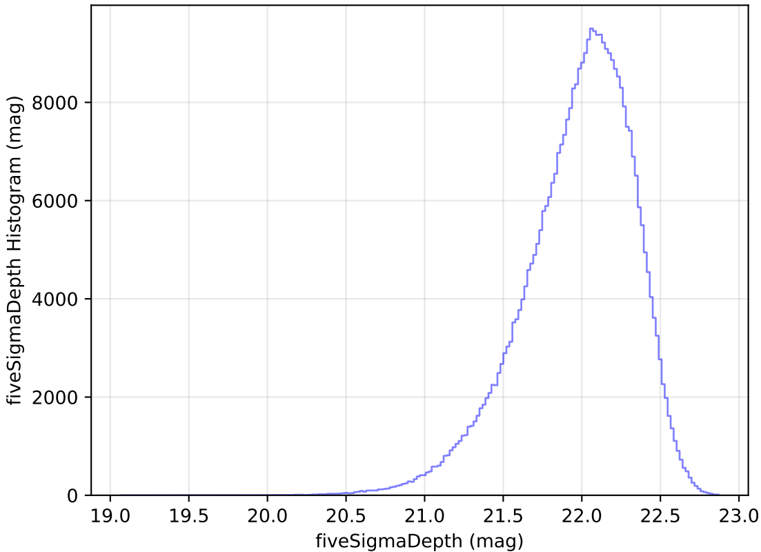
ddf_loaded_fl8_v3.4_10yrs y: fiveSigmaDepth Histogram
