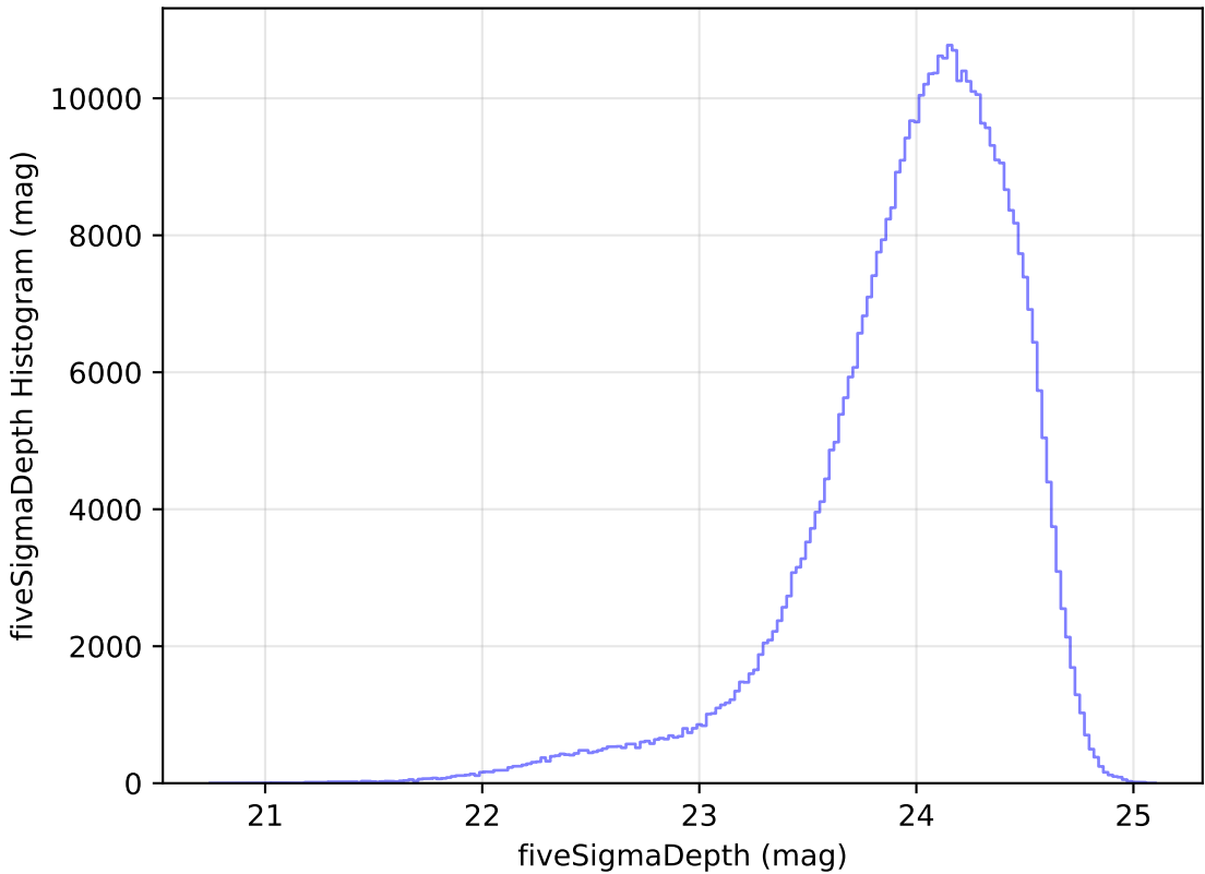
ddf_loaded_fl8_v3.4_10yrs r: fiveSigmaDepth Histogram
