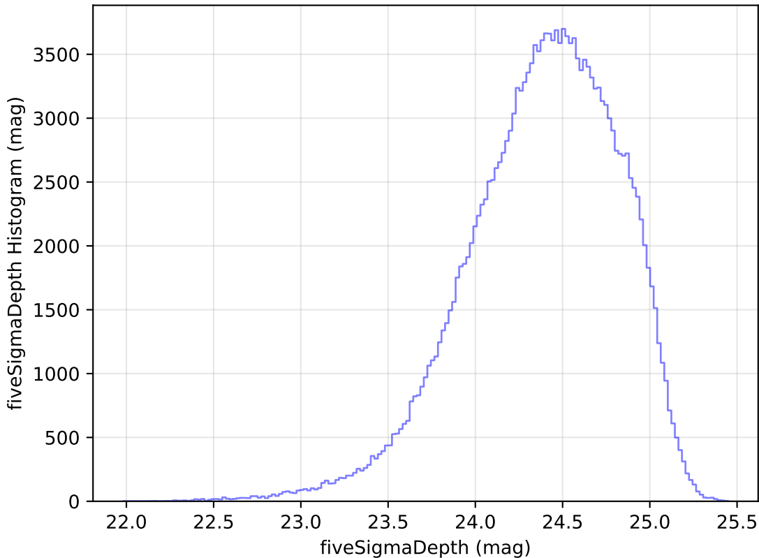
ddf_loaded_fl8_v3.4_10yrs g: fiveSigmaDepth Histogram
