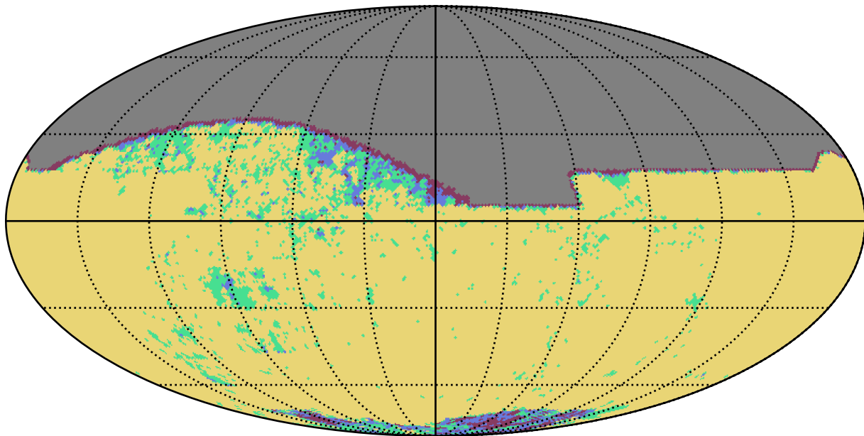
ddf_loaded_fl8_v3.4_10yrs z band: YearCoverage night
