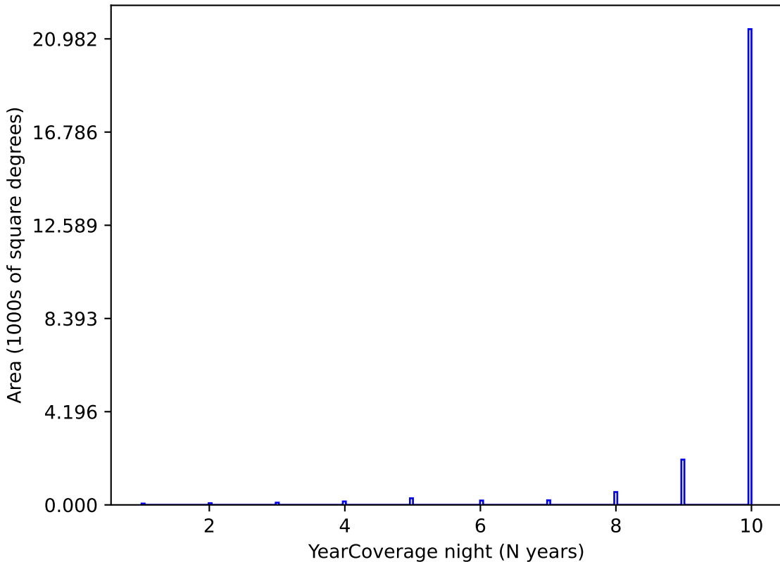
ddf_loaded_fl8_v3.4_10yrs y band: YearCoverage night
