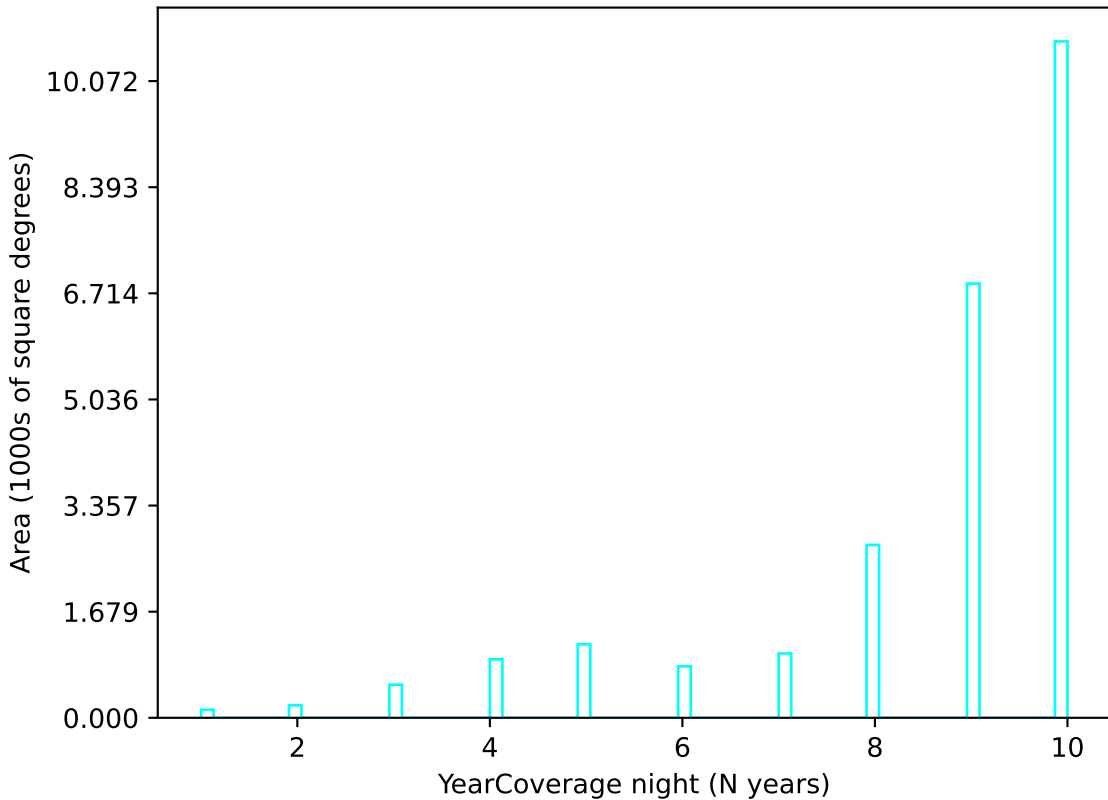
ddf_loaded_fl8_v3.4_10yrs u band: YearCoverage night
