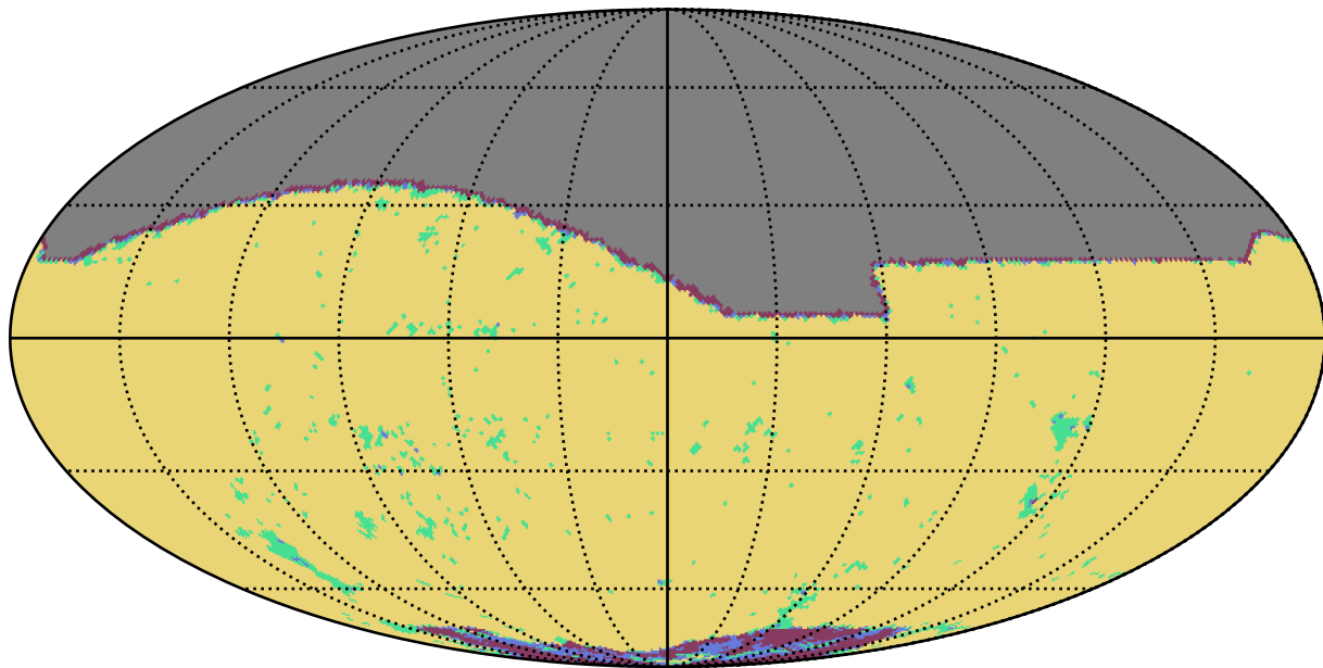
ddf_loaded_fl8_v3.4_10yrs r band: YearCoverage night
