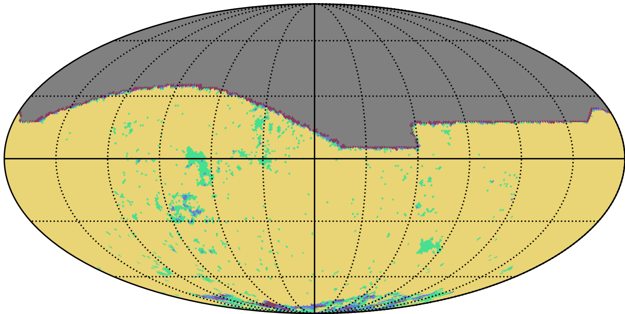
ddf_loaded_fl8_v3.4_10yrs i band: YearCoverage night
