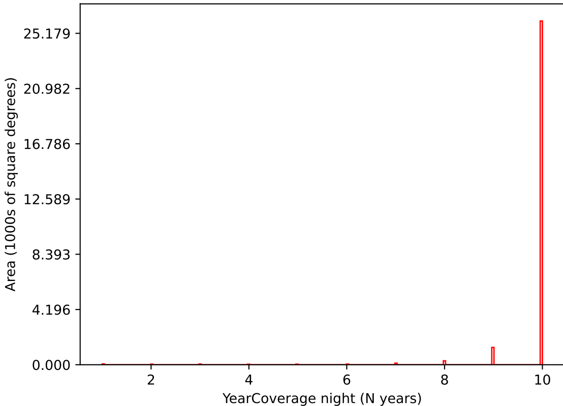
ddf_loaded_fl8_v3.4_10yrs i band: YearCoverage night
