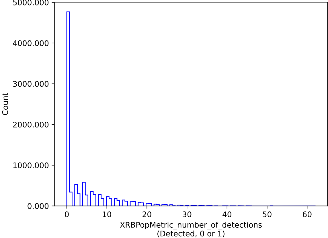
ddf_loaded_fl8_v3.4_10yrs : XRBPoMetric_number_of_detections
