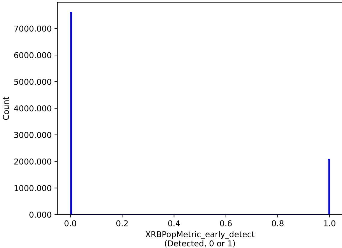
ddf_loaded_fl8_v3.4_10yrs : XRBPoMetric_early_detect
