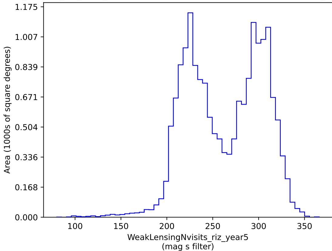
ddf_loaded_fl8_v3.4_10yrs gri band non-DD: WeakLensingNvisits_riz_year5
