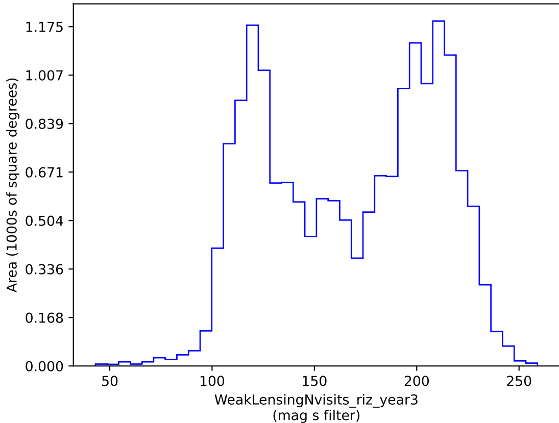
ddf_loaded_fl8_v3.4_10yrs gri band non-DD: WeakLensingNvisits_riz_year3
