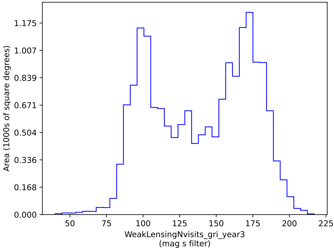
ddf_loaded_fl8_v3.4_10yrs gri band non-DD: WeakLensingNvisits_gri_year3
