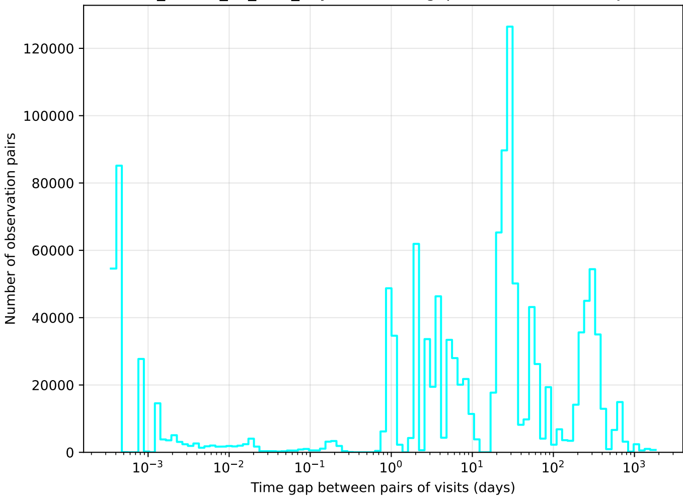
ddf_loaded_fl8_v3.4_10yrs u band: Tgaps observationStartMJD
