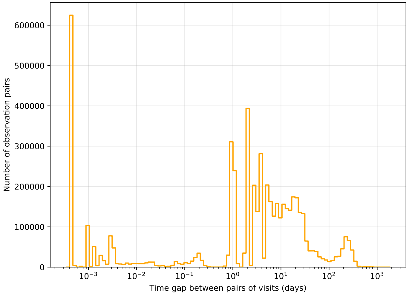
ddf_loaded_fl8_v3.4_10yrs r band: Tgaps observationStartMJD
