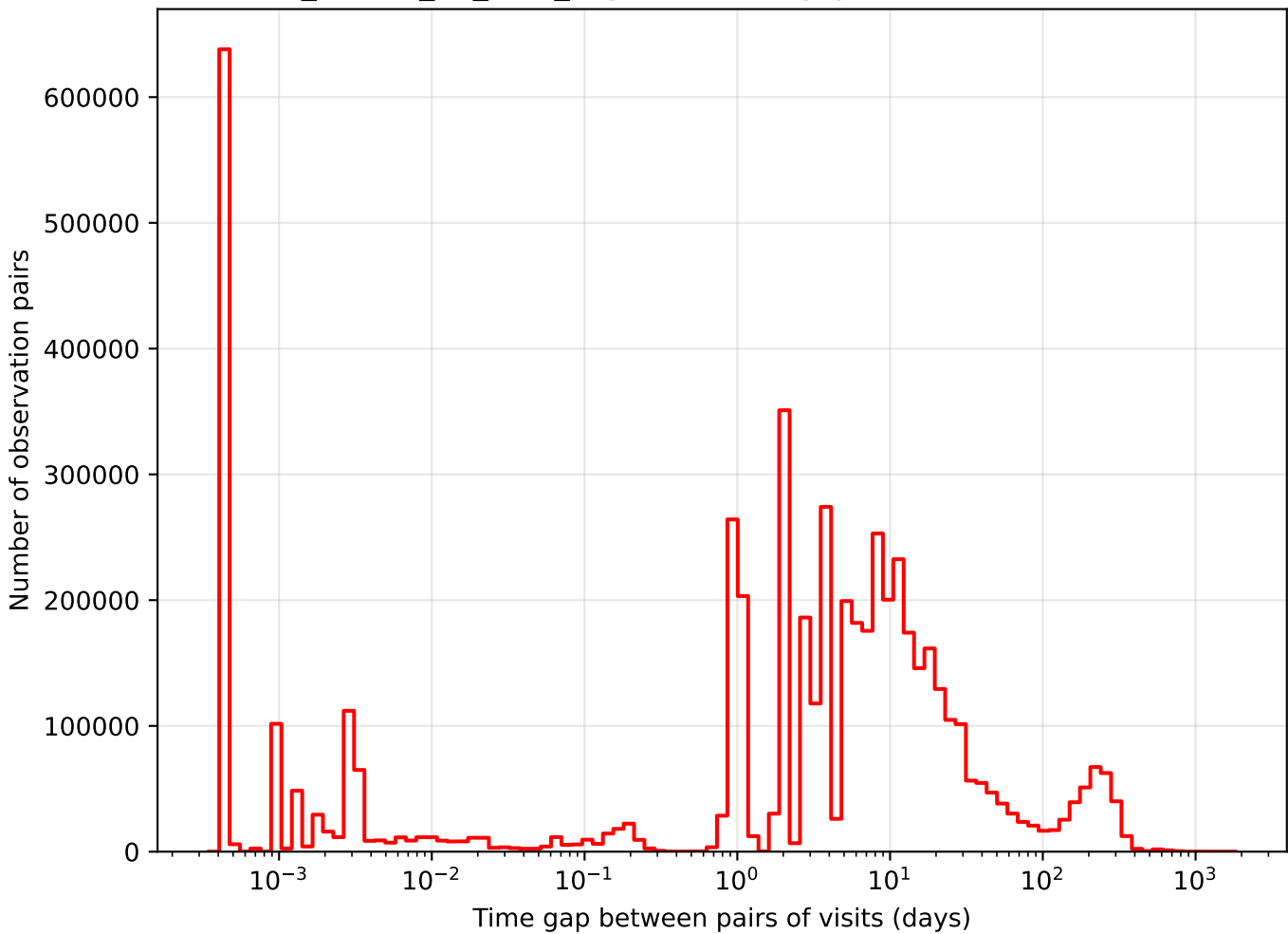
ddf_loaded_fl8_v3.4_10yrs i band: Tgaps observationStartMJD
