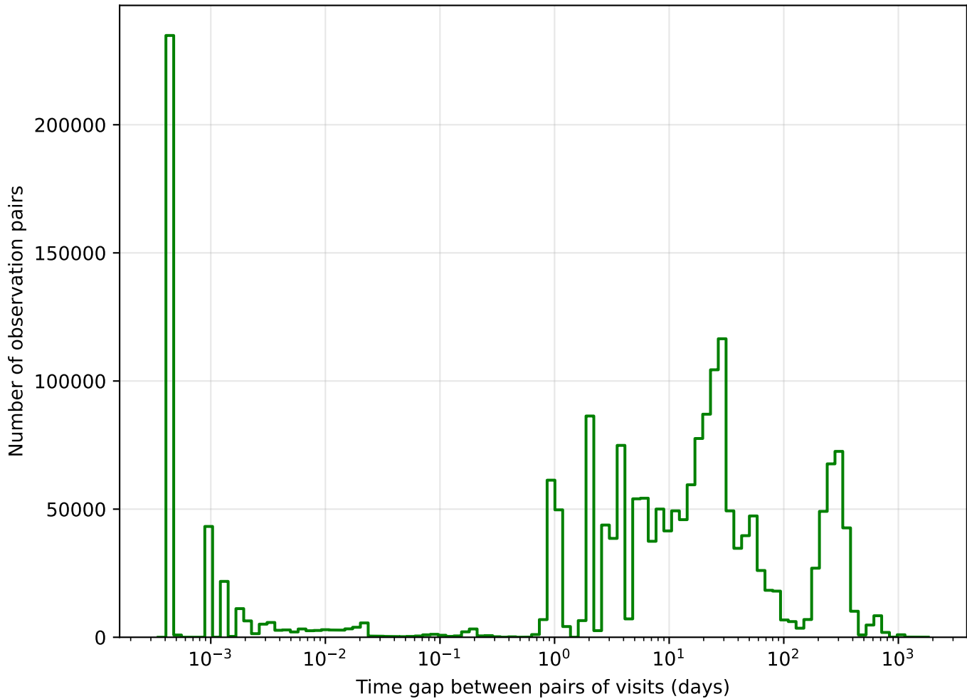
ddf_loaded_fl8_v3.4_10yrs g band: Tgaps observationStartMJD
