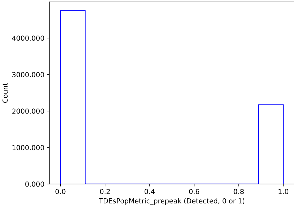
ddf_loaded_fl8_v3.4_10yrs : TDEsPopMetric_prepeak
