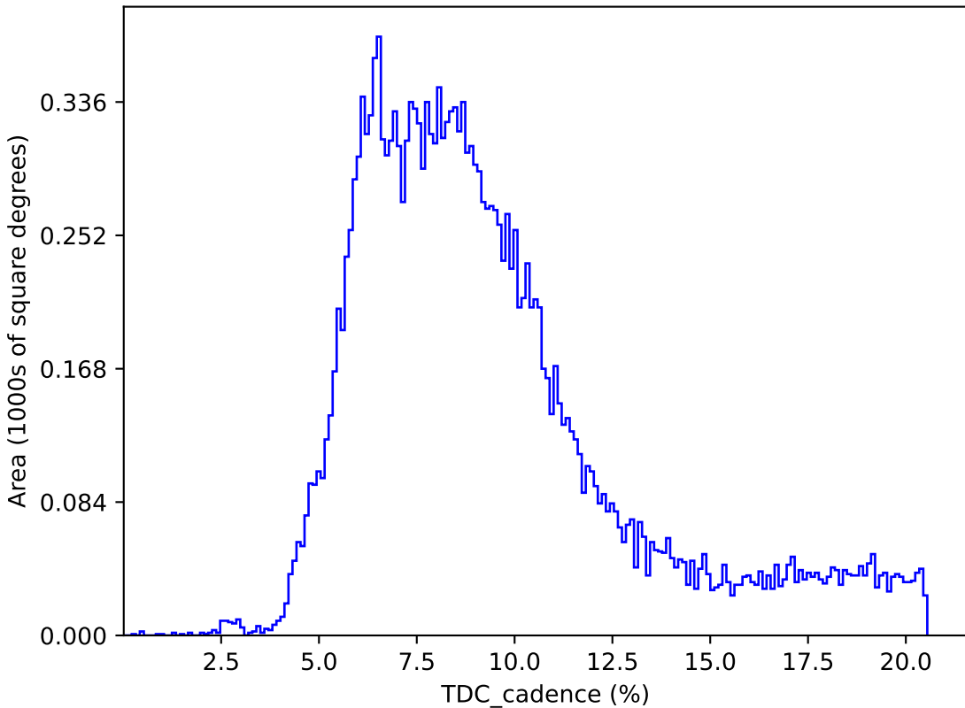
ddf_loaded_fl8_v3.4_10yrs : TDC_cadence
