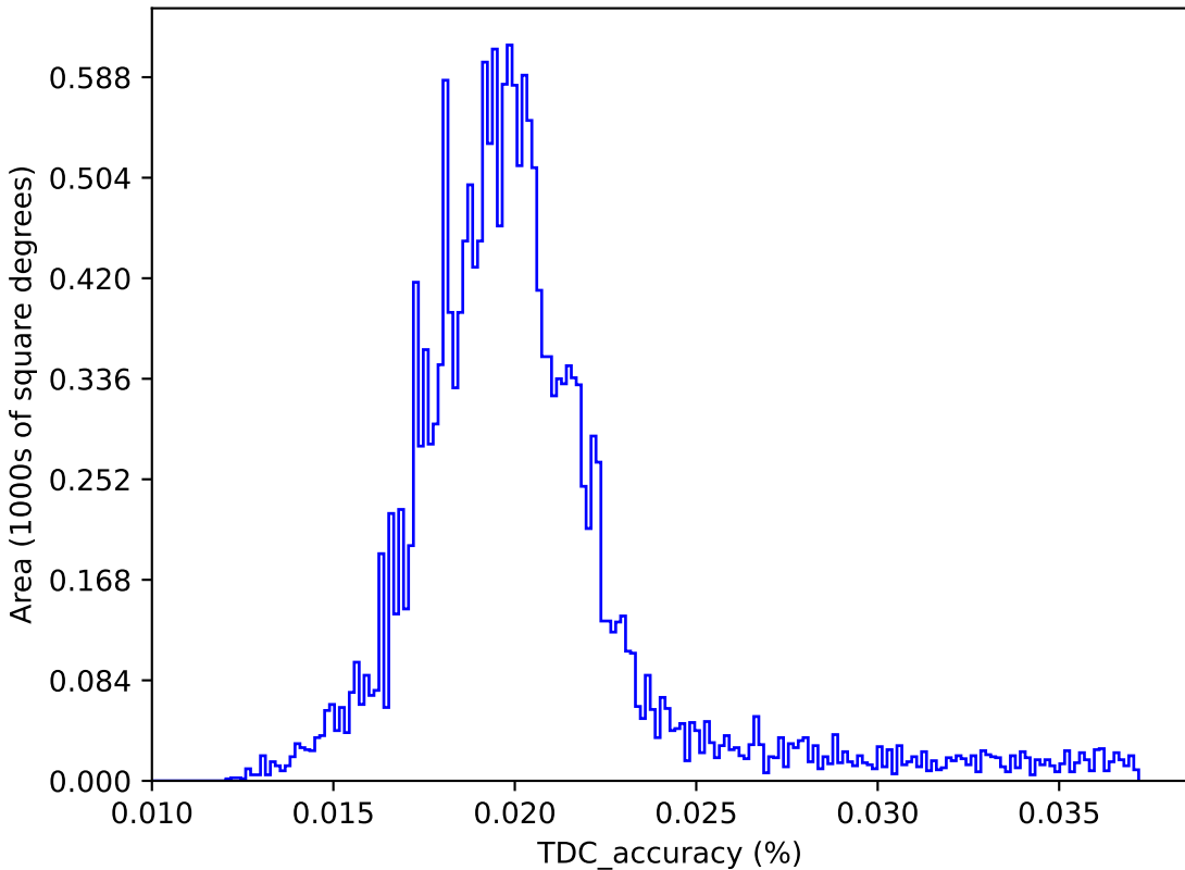
ddf_loaded_fl8_v3.4_10yrs : TDC_accuracy
