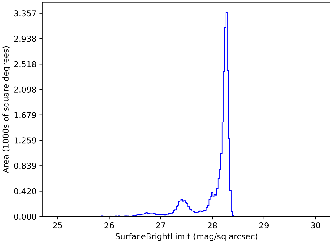
ddf_loaded_fl8_v3.4_10yrs y: SurfaceBrightLimit
