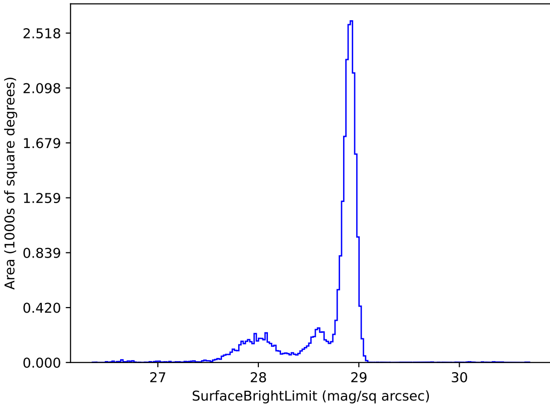
ddf_loaded_fl8_v3.4_10yrs u: SurfaceBrightLimit
