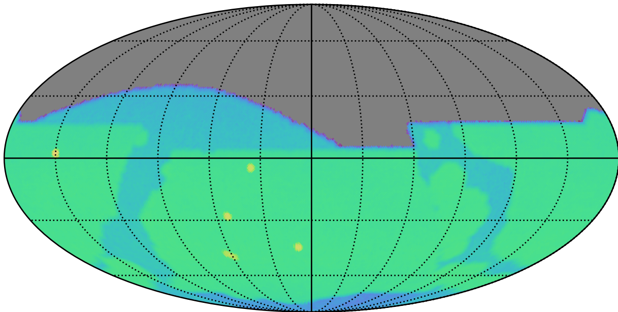
ddf_loaded_fl8_v3.4_10yrs r: SurfaceBrightLimit
