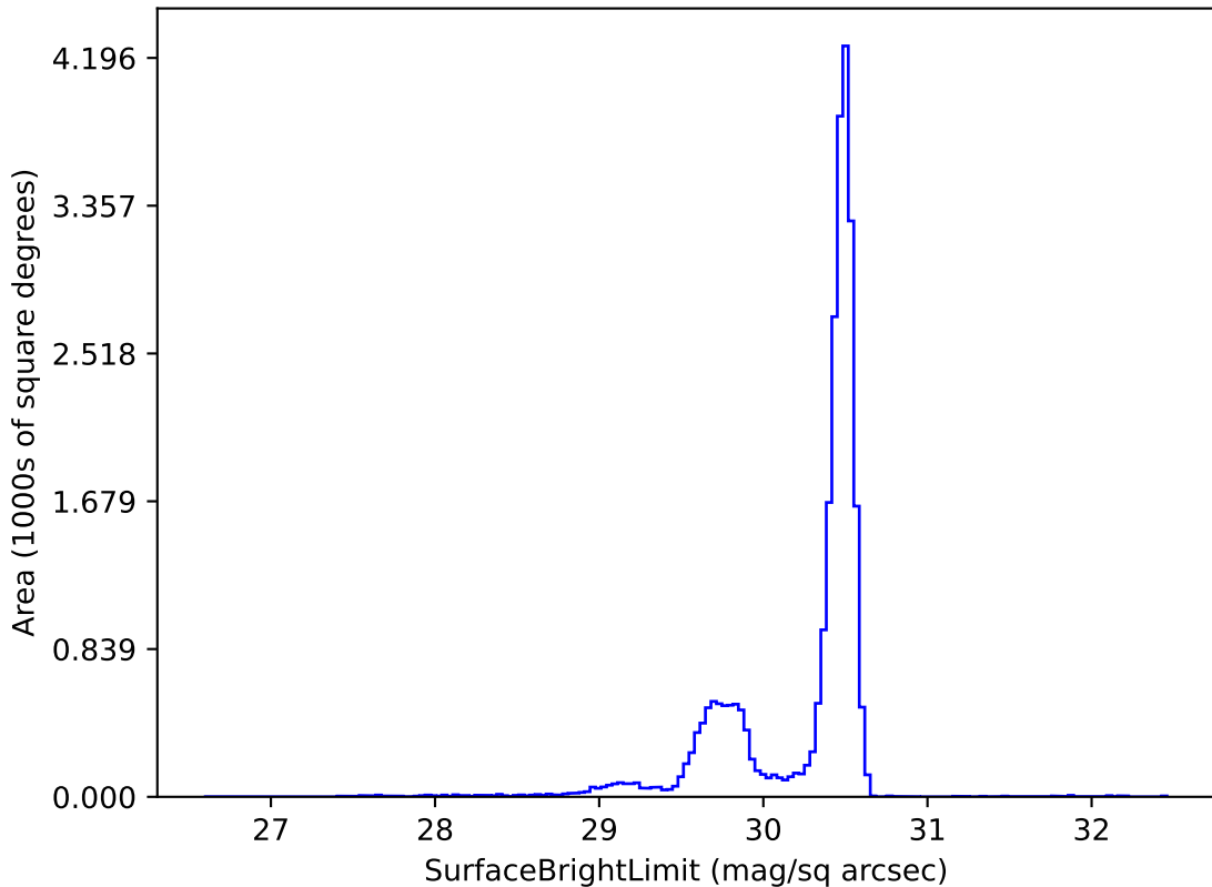
ddf_loaded_fl8_v3.4_10yrs r: SurfaceBrightLimit
