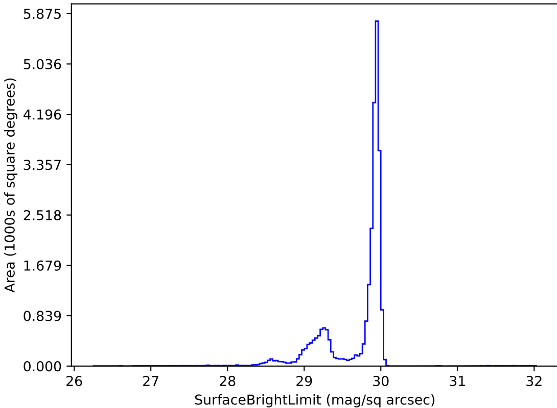
ddf_loaded_fl8_v3.4_10yrs i: SurfaceBrightLimit
