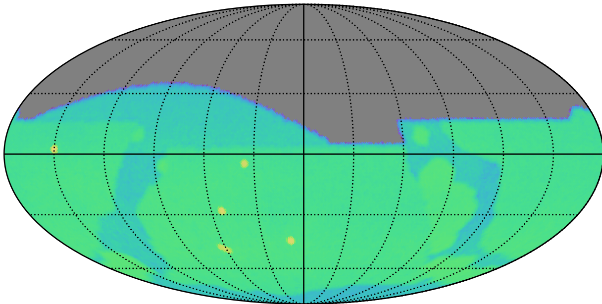
ddf_loaded_fl8_v3.4_10yrs g: SurfaceBrightLimit
