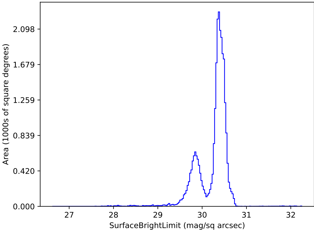
ddf_loaded_fl8_v3.4_10yrs g: SurfaceBrightLimit
