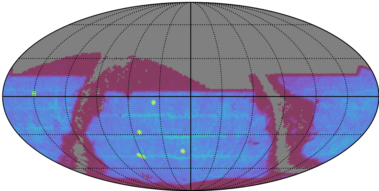
ddf_loaded_fl8_v3.4_10yrs : SNSLMetric
