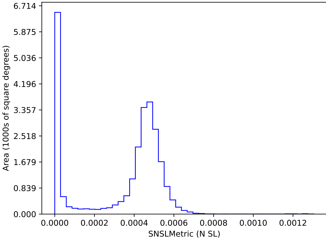
ddf_loaded_fl8_v3.4_10yrs : SNSLMetric
